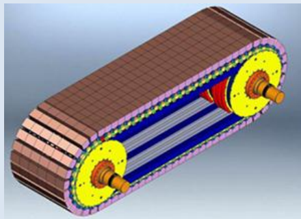
Segmented Copper Casting Blocks
